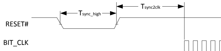
Figure 5-44. AC97 Warm Reset Timing
