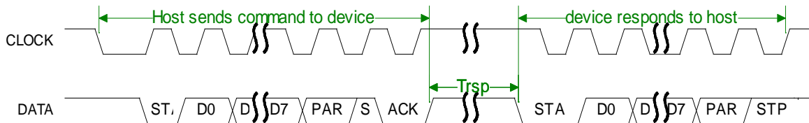
Figure 5-34. PS2 Timing for Master Sending Command then Device Sending Response
