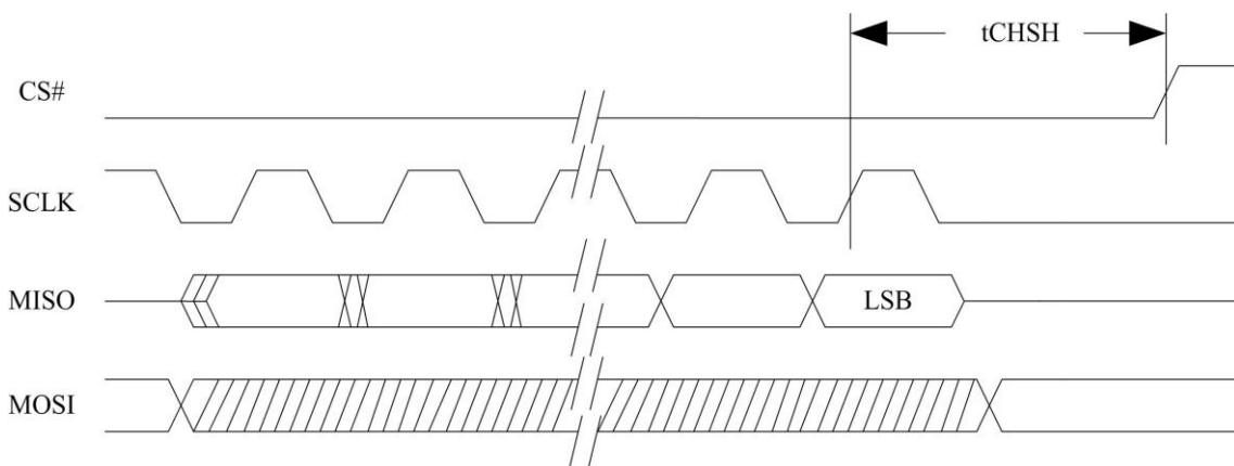
Figure 5-37. SPI MISO Timing
