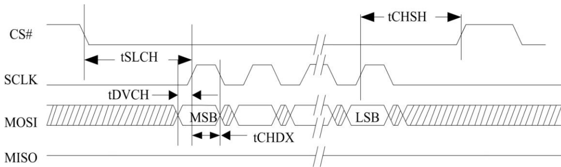
Figure 5-36. SPI MOSI Timing
