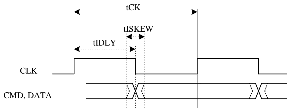
Figure 5-22. SMHC in SDR Mode Input Timing
