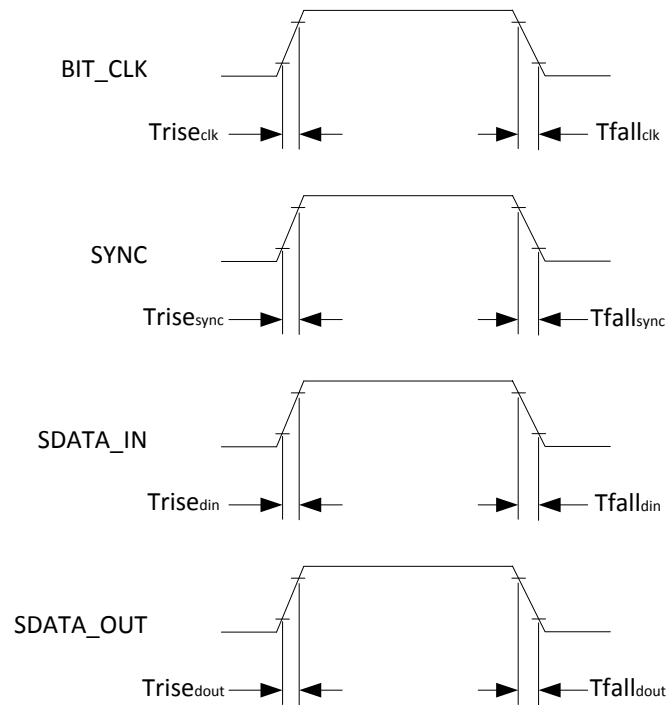
Figure 5-48. Signal Rise and Fall Timing
