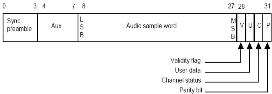
Figure 7-14. Sub-Frame Format
